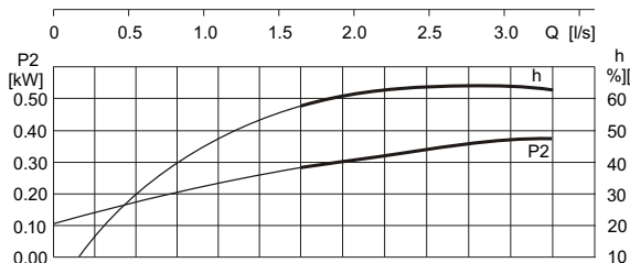
Performance curves are given according to ISO9906: 2012 Gr3B.
