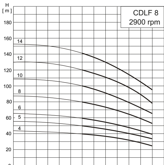
Performance curves are given according to ISO9906: 2012 Gr3B.
